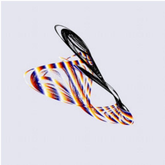
reb-Slope_3D_Quadratic_G_Attractor-02.jp
