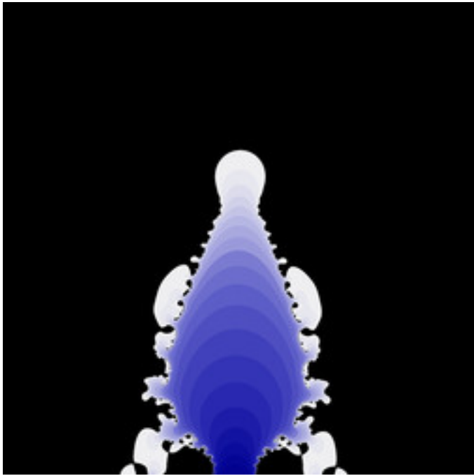
dmj-StutterMandel-03.jpg
