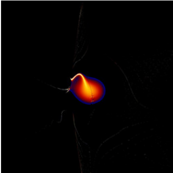
mt-zeepop-mset-51.jpg
