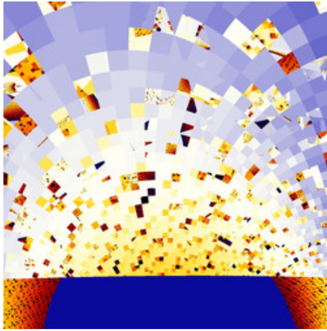
mt-biomorphIMset-10.jpg
