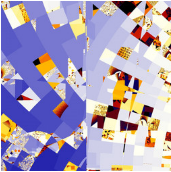
mt-biomorphIMset-11.jpg
