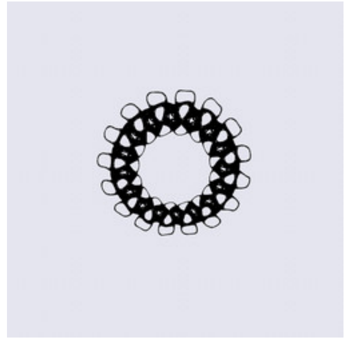
reb-Slope_4D_Special_Map_#2_G_Attractor-
