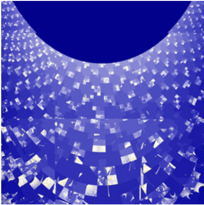
mt-biomorphIMset-05.jpg
