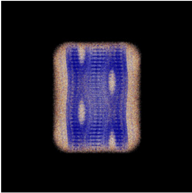
mt-latoocarfian-ii-34.jpg
