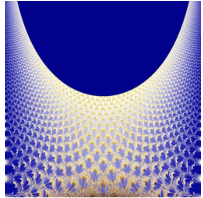
mt-biomorphIMset-03.jpg
