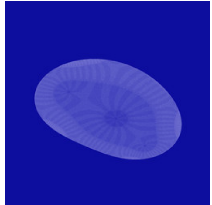
reb-4DMagnet13RDIMJulia-02.jpg
