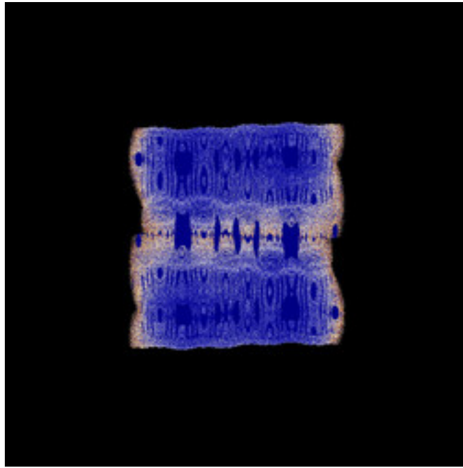
mt-latoocarfian-ii-33.jpg
