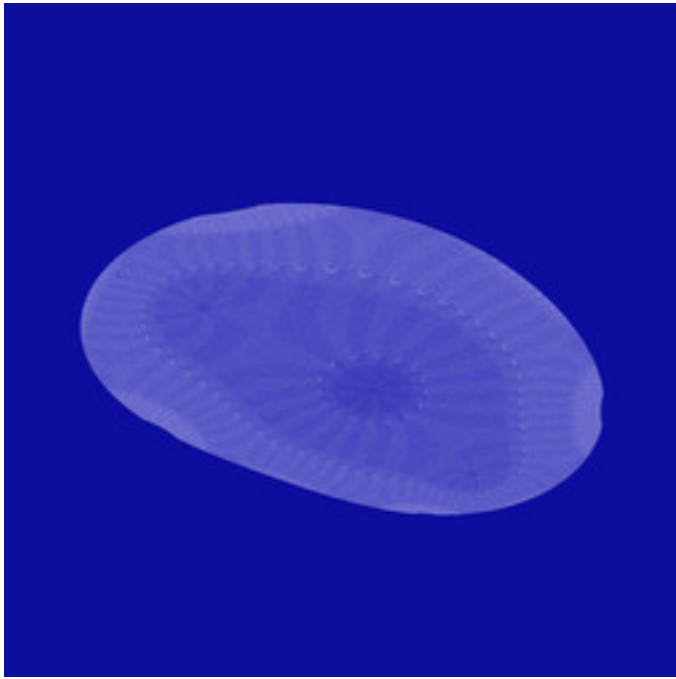
reb-4DMagnet13RDIMJulia-01.jpg
