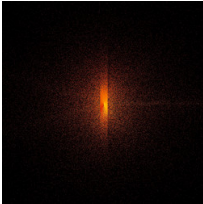
mt-newton-twist-13.jpg
