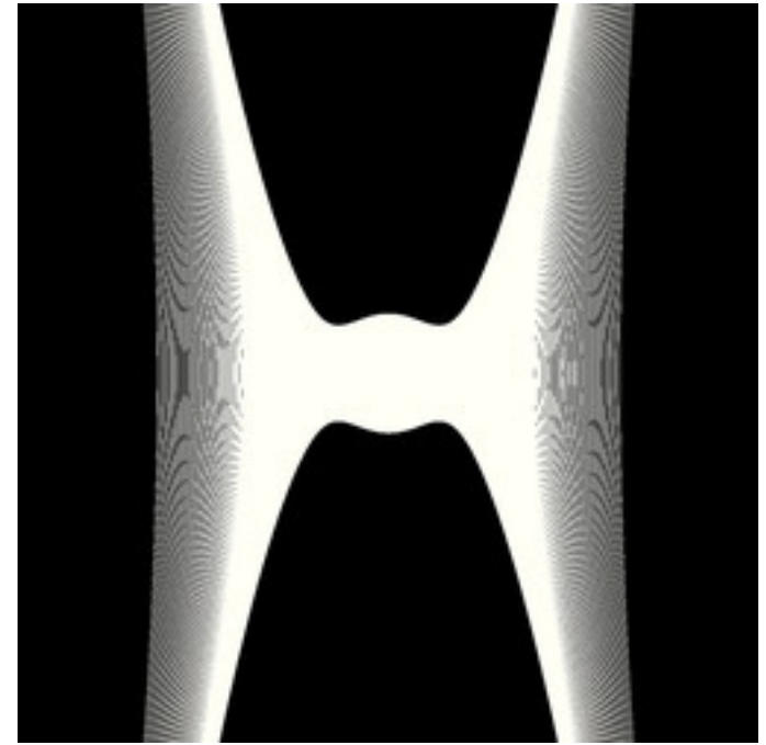
reb-FormulaTracer-11A.jpg
