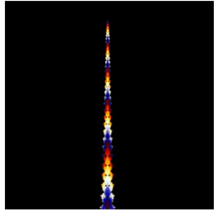
dmj-StutterMandel-01.jpg
