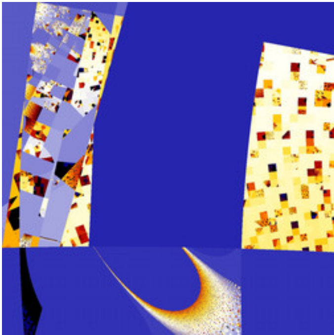
mt-biomorphIMset-14.jpg
