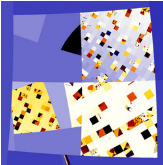
mt-biomorphIMset-13.jpg
