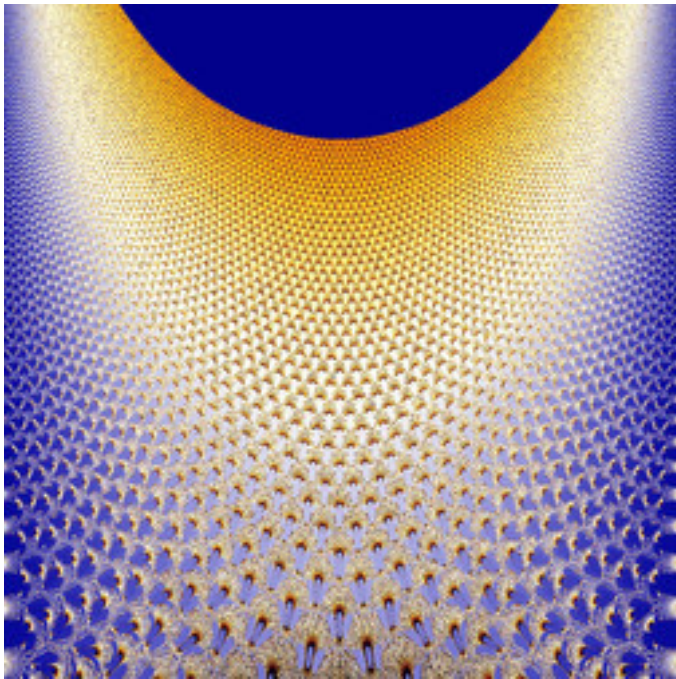
mt-biomorphIMset-02.jpg
