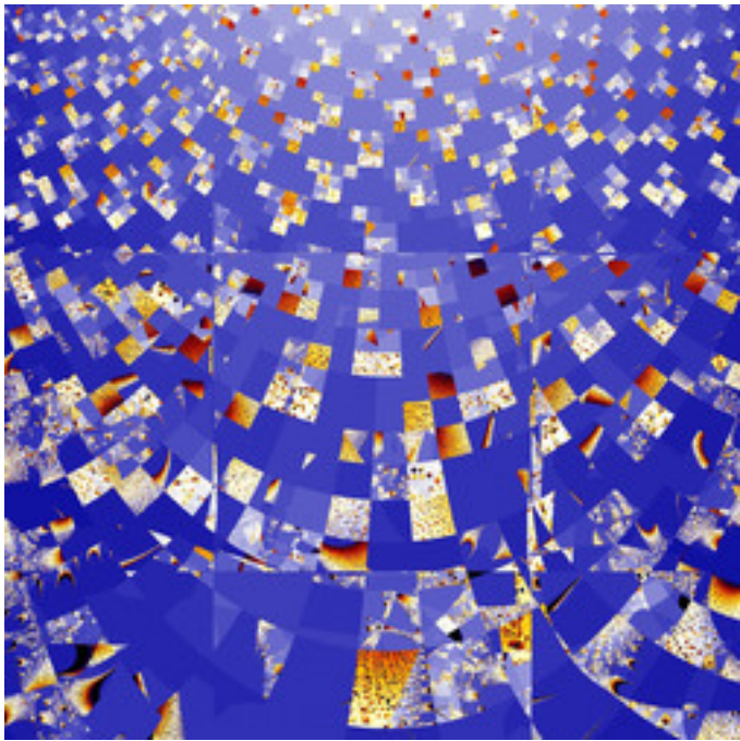
mt-biomorphIMset-08.jpg
