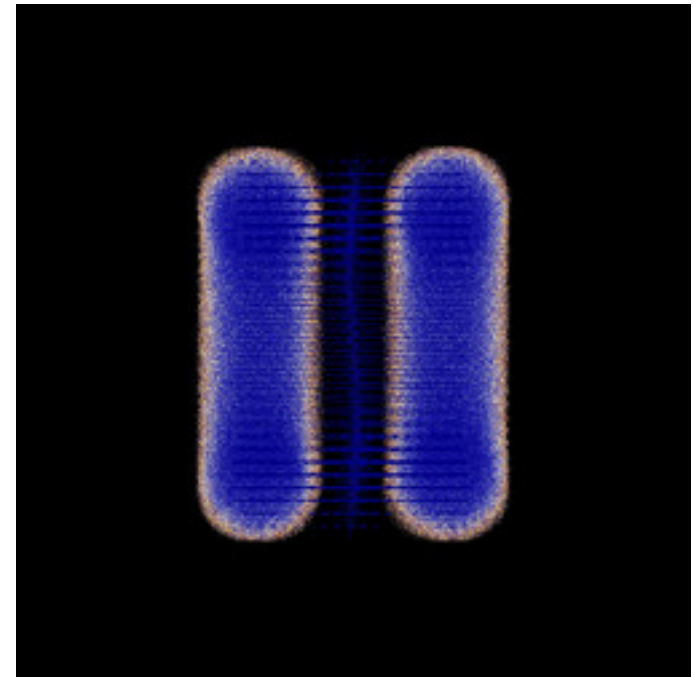
mt-latoocarfian-ii-35.jpg
