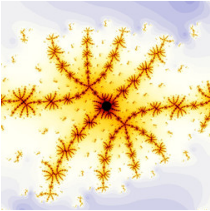
lkm3-CompoundMandelbrot-01.jpg
