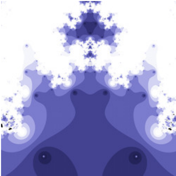
dmj-DoubleHalleyNova-01.jpg
