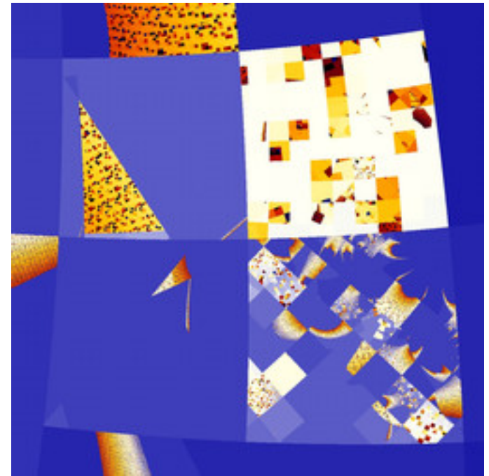
mt-biomorphIMset-12.jpg
